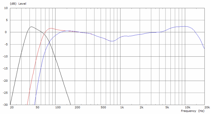
LS118 and LA112 frequency responses, on-axis at 1 m.
