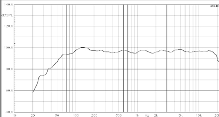
Frequency response
