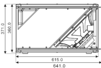
Front
